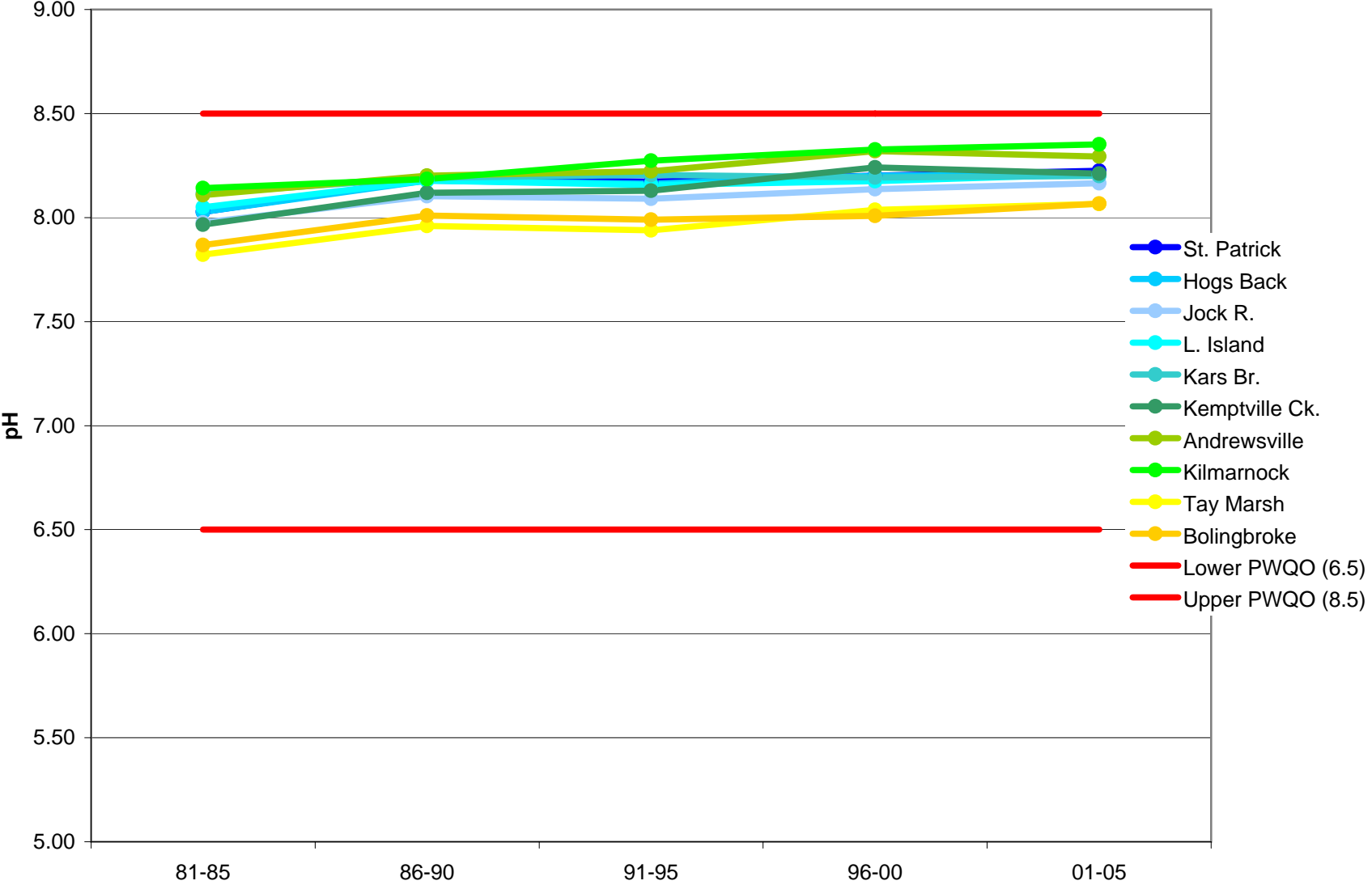
pH - 5 Year Geometric Mean Concentrations
