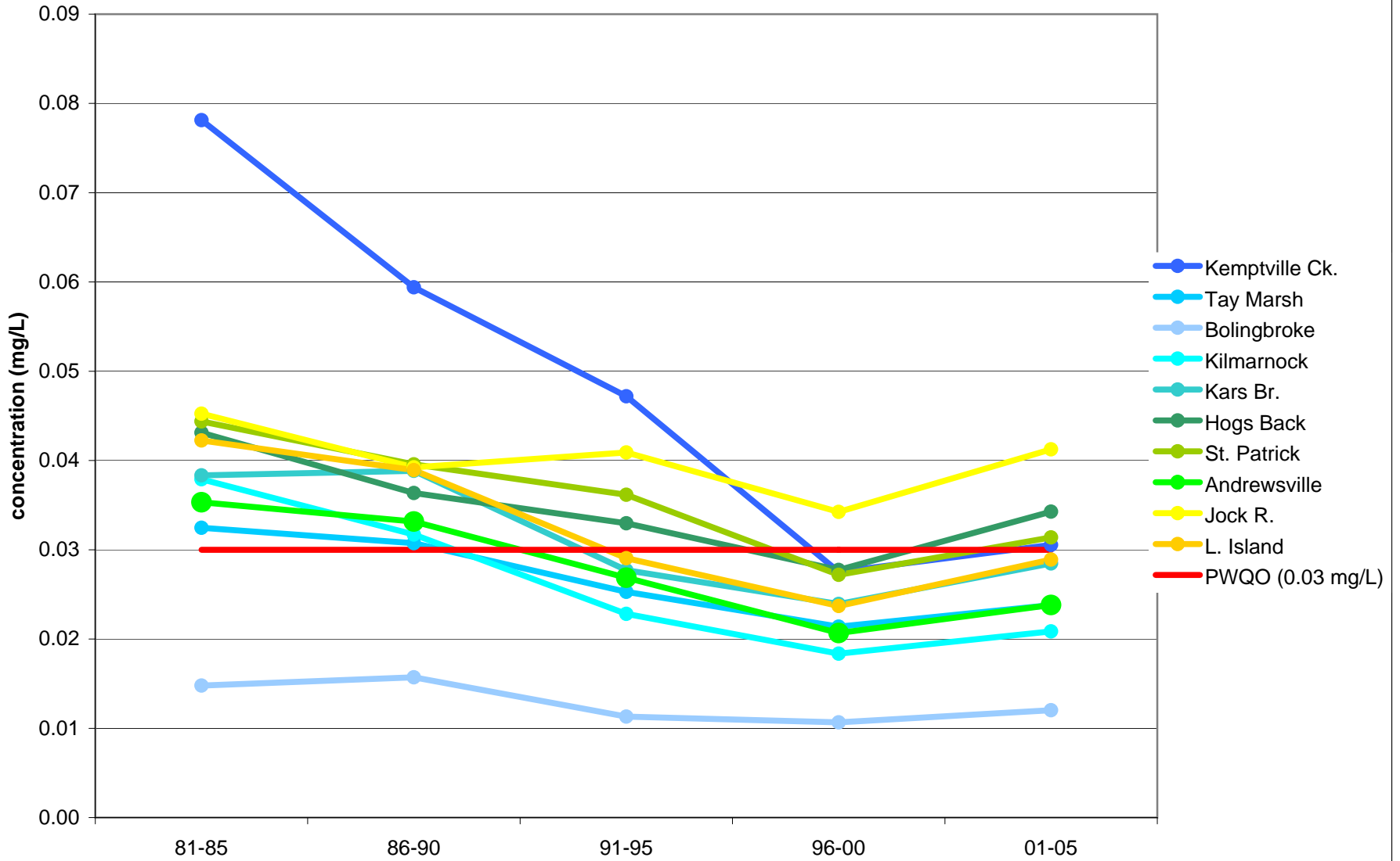
Total Phosphorus - 5 Year Geometric Mean Concentrations
