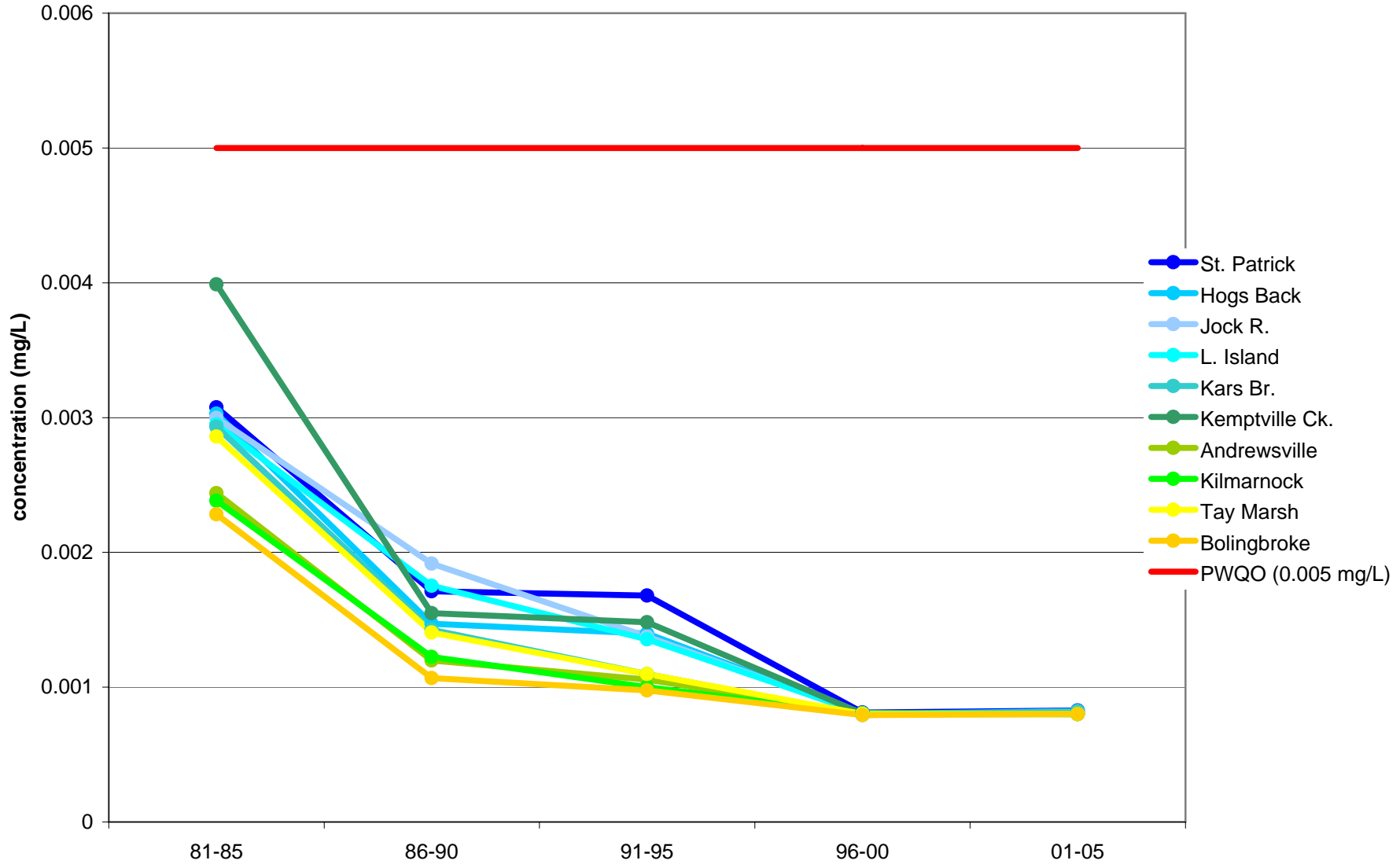
Copper - 5 Year Geometric Mean Concentrations
