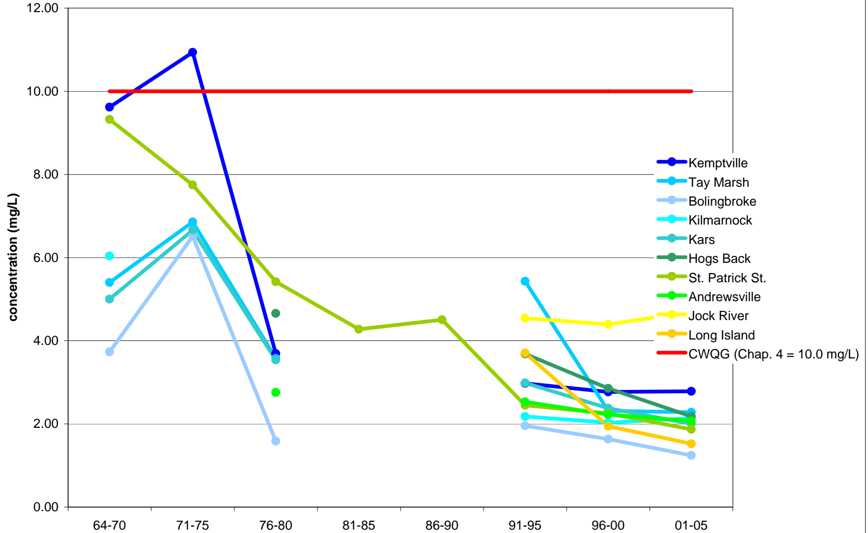
TSS - 5 Year Geometric Mean Concentrations
