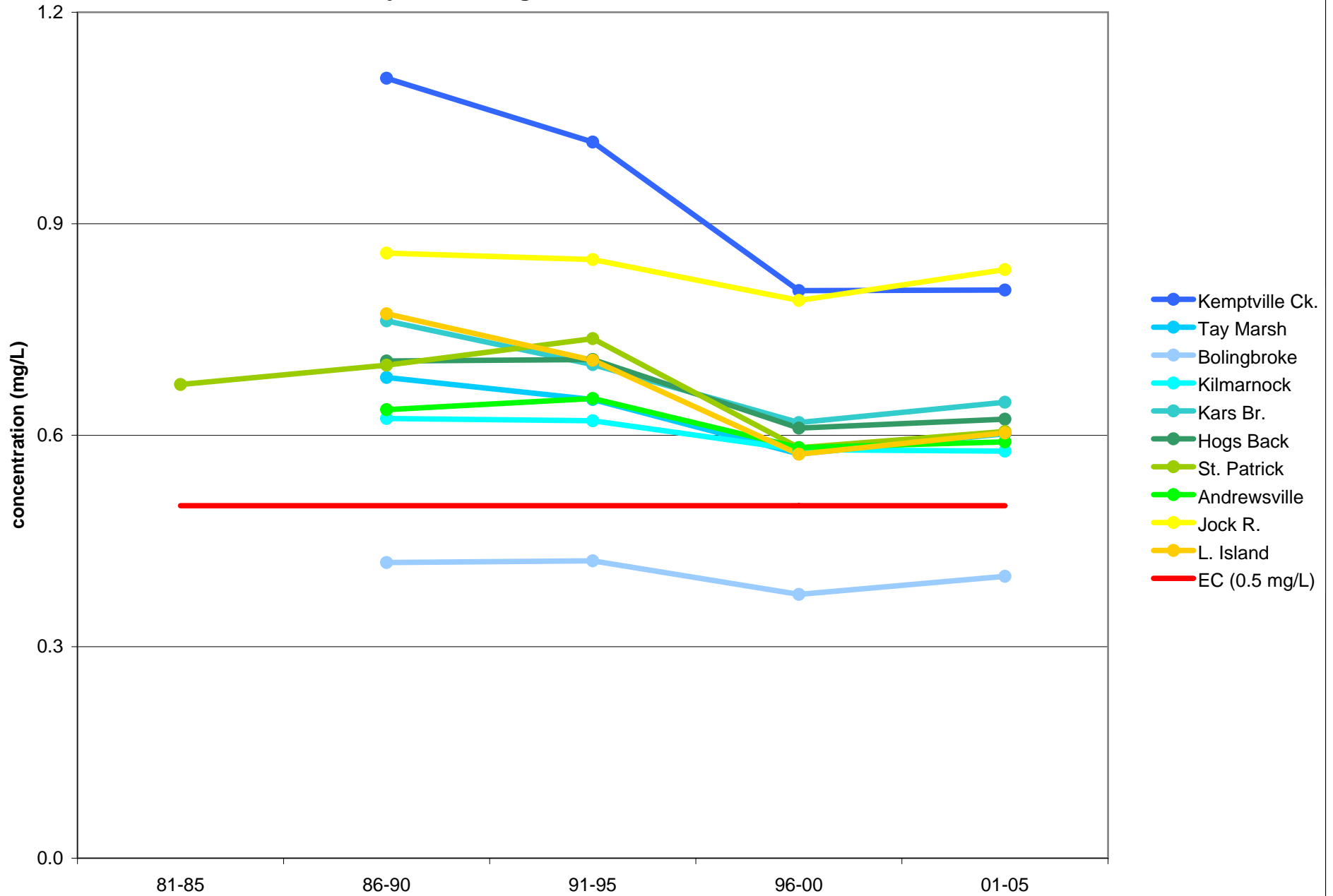
Total Kjeldahl Nitrogen - 5 Year Geometric Mean Concentrations
