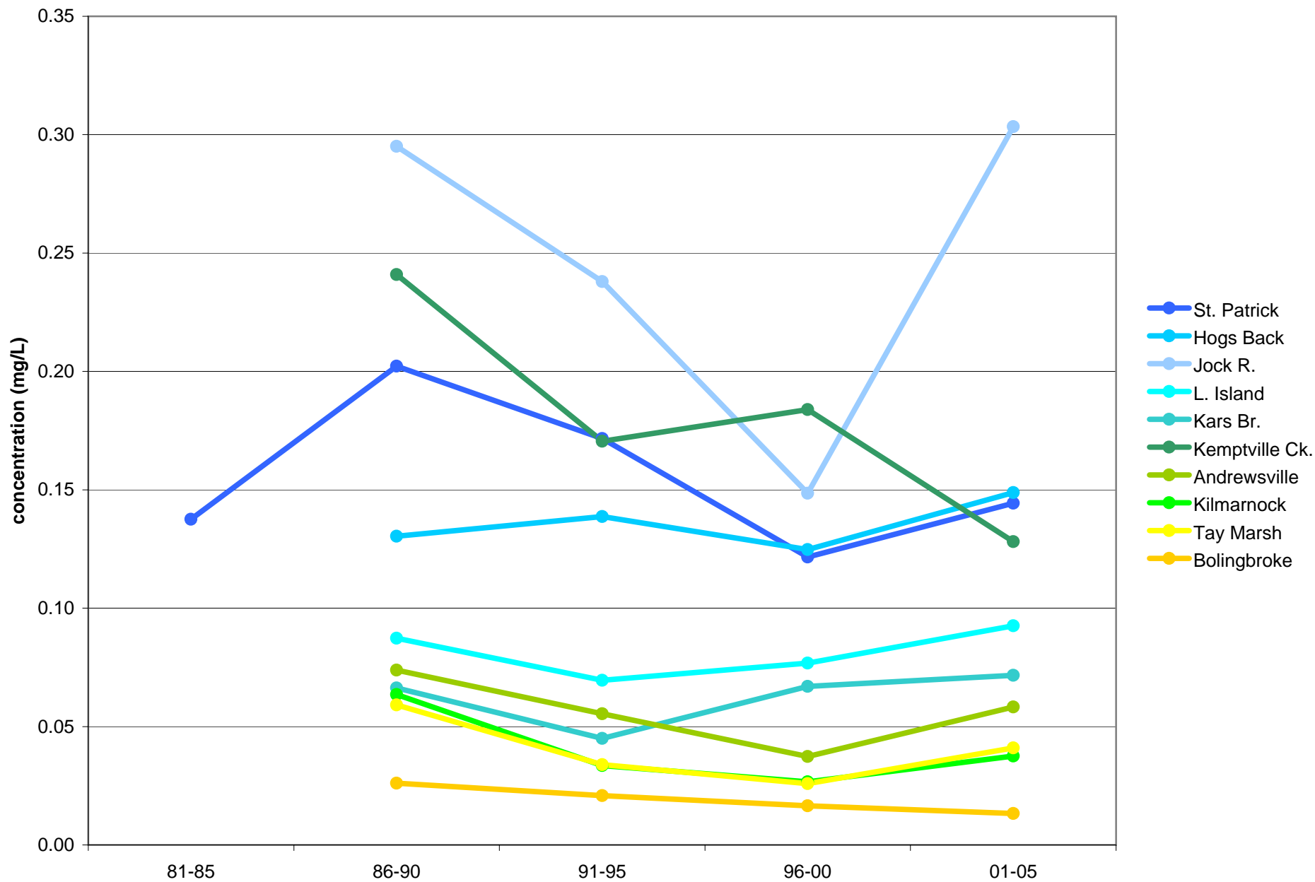
Nitrates - 5 Year Geometric Mean Concentrations
